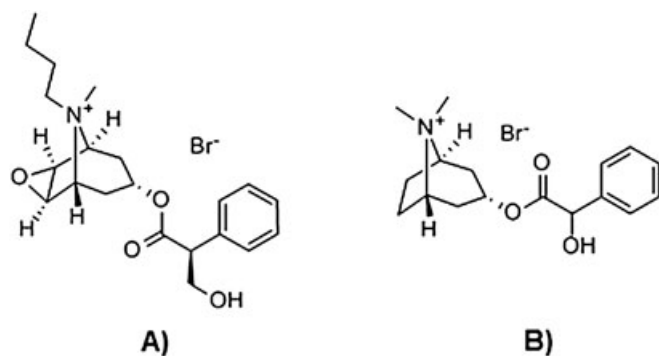
Figure 1. Chemical structure of (A) N-butylscopolamine bromide and (B) N-methylhomatropine bromide.
